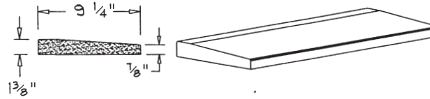
#TH-51 (1/2" SLOPE)
