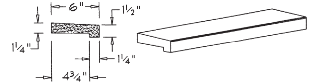
#TH-100 (1/4" SLOPE)
