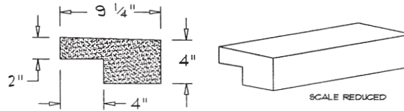
#TH-102 (1/4" SLOPE)
