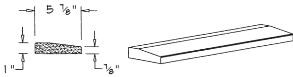
#TH-50 (1/2" SLOPE)
