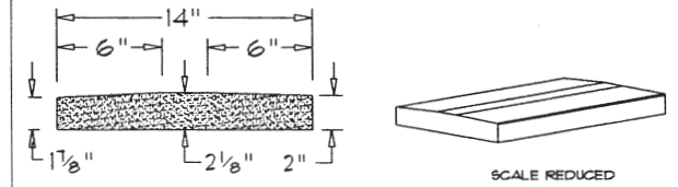
#TH-103 @ 36" (1/4" SLOPE RT., 1/8" SLOPE LT.)
