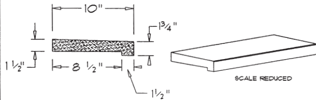
#TH-101 (1/4" SLOPE)
