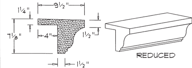
SL-222 (@ 30", 1/4" SLOPE)
