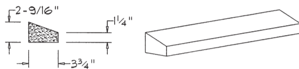
SL-225 (1-5/16" SLOPE)
