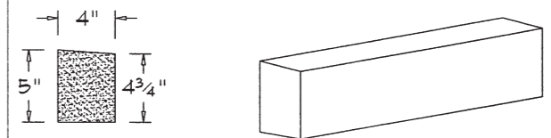
SL-213 ( 1/4" SLOPE)
