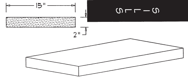
SL-244 ( @ 30" )
