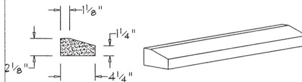
SL-226 (1/8" SLOPE)
