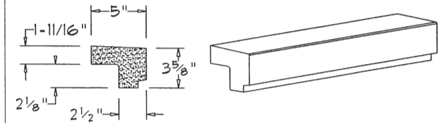
SL-219 (3/16" SLOPE)
