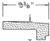
SL-248 — CONTINUOUS DRIP
