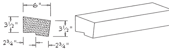
SL-218 (1/8" SLOPE)
