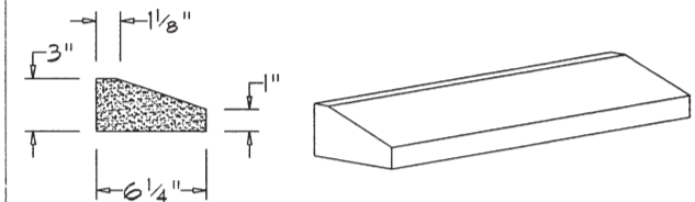
SL-227 (1 3/4" SLOPE)
