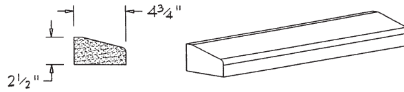
SL-231 (1" SLOPE)
