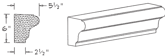
SL-204 ( 1/8" SLOPE)
