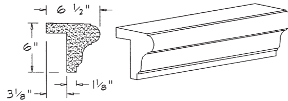
SL-205 ( 1/8" SLOPE)
