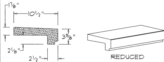
SL-220 (3/8" SLOPE)
