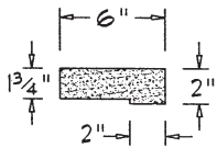
SL-245 ( @ 30" ) — CONTINUOUS DRIP
