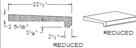
SL-221 (SLOPE: 1/2"/FT.)
