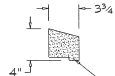
SL-251 — CONTINUOUS DRIP
